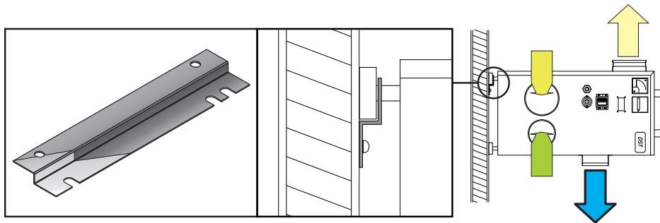
FIGURE 10: Bracket for wall mount
