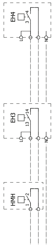
Optional Humidistat, connection examples
